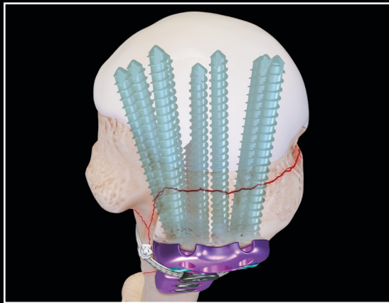
Low-profile plate with divergent screw pattern
